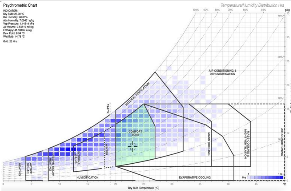
Figure 4: Givoni Bioclimatic chart for the climate of Mascalucia using Andrew Marsh online tool. Climate data are extracted from http://climate.onebuilding.org/WMO_Regio_6_Europe/ITA_Italy/SC_Sicily/ITA_SC_Catania.Fontanarossa.AP.164600_TMYx.2004-2018.zip [8]
