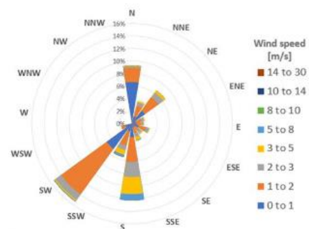
Figure 6: Wind rose for Mascalucia [4]
